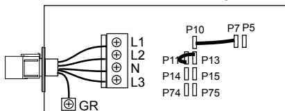
3-Phase Connection with Single Neutral
