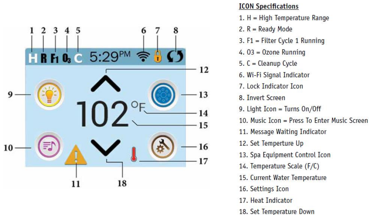
Figure 15. Main Screen Layout
