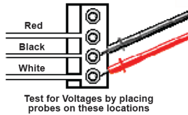
Figure 2. Proper Voltage Readings Across Terminals on House Breaker Box, Swim Spa and Exercise Pool System Box and GFCI
